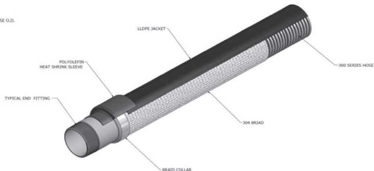
Figure 2 - Typical Hose Assembly with End Fitting
