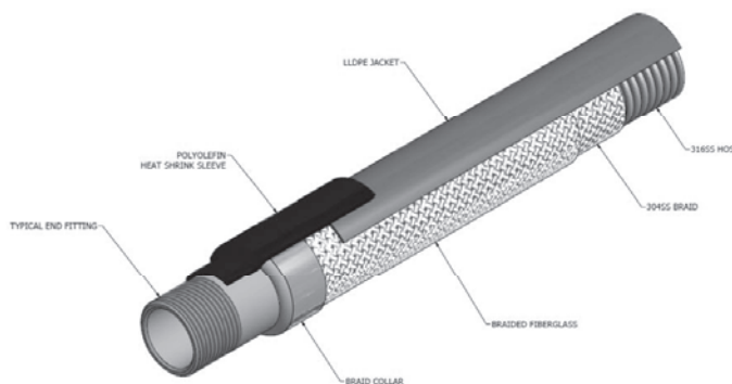
Figure 2 - Typical Hose Assembly with End Fitting
